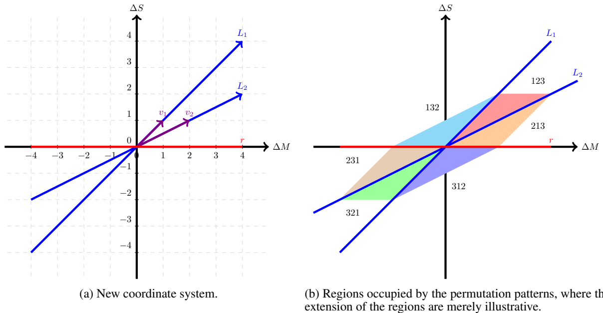
Figure 3. Regions in the \Delta M \times \Delta S plane in terms of T_{MS} .
