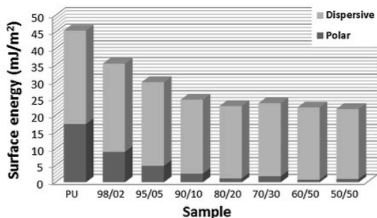
Fig. 5 Surface energies of PU/nanoPTFE composites
