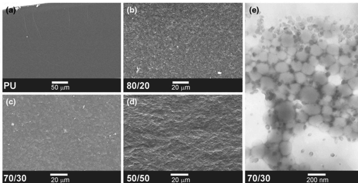
Fig. 6 SEM images for PU (a), 80/20 (b), 70/30 (c), 50/50 (d), and TEM image for 70/30 (e)
