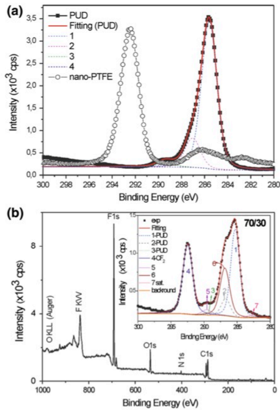
Fig. 2 a XPS spectra of C1s peak for pure PU and nanoPTFE. b Survey XPS spectra of B70:30 sample. Inset graph shows the C1s fitted components The peak label 7 is an X-ray satellite of component 4 (see text for details)
