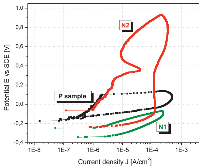
Fig. 5. Cyclic polarization curves of nitrated samples and aged PH sample.
